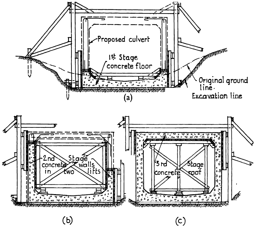
Fig. 331.—Shuttering for Box Culverts.
